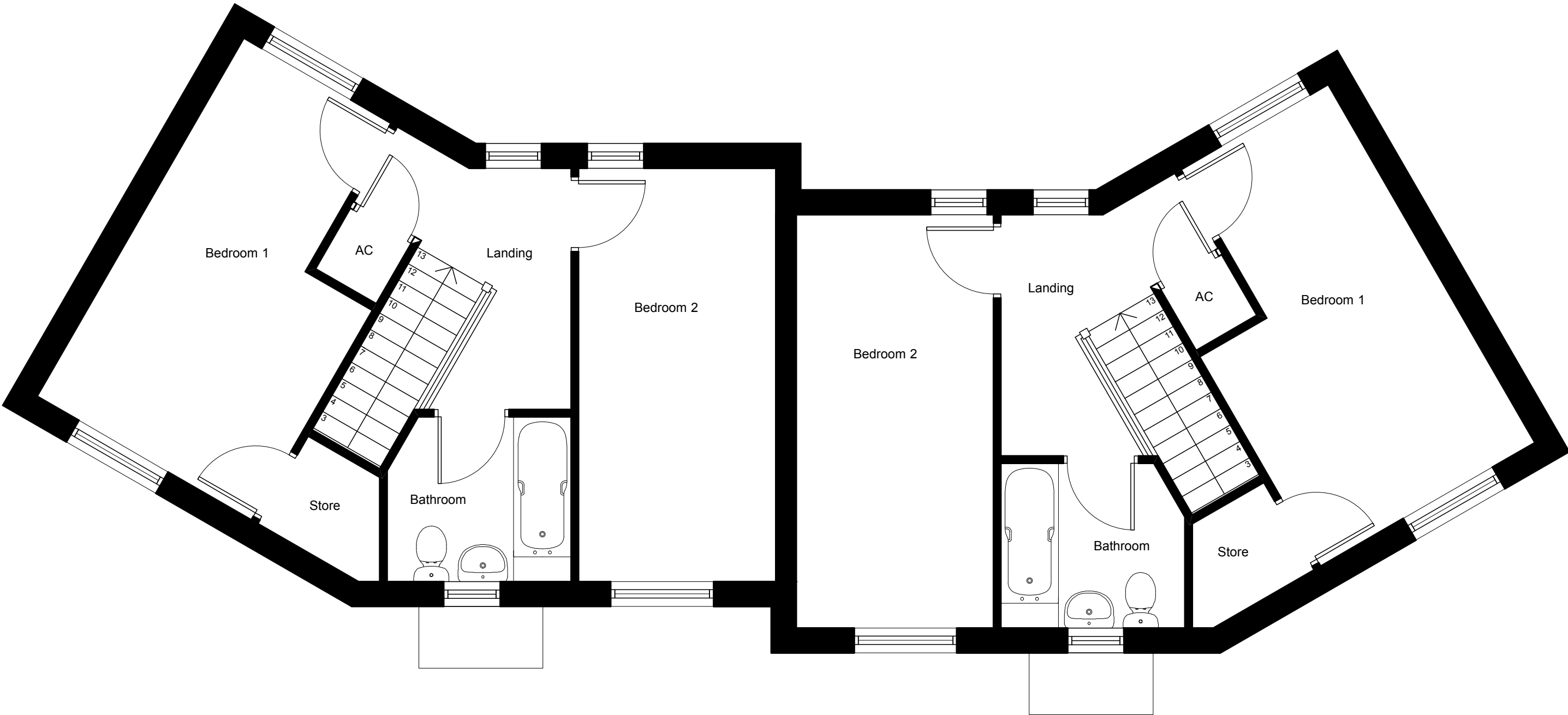
First Floor Plan Plots 19-20
